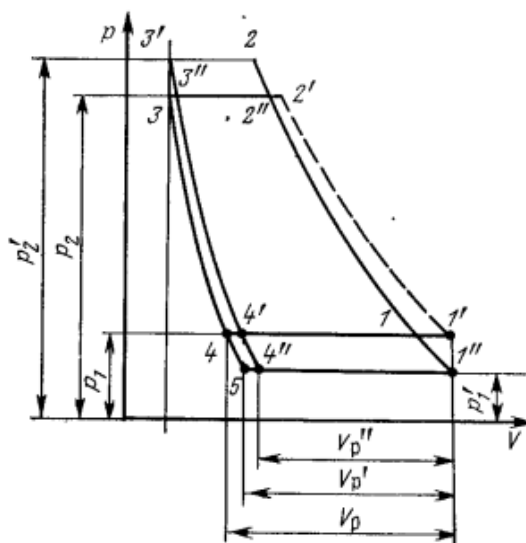
1 – rasm. Kompessor silindrida havoni so‘rish, siqish va haydash jarayonining indikator diagrammasi
